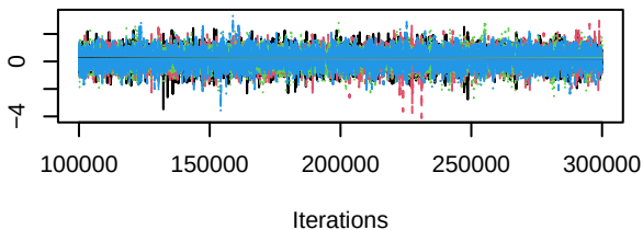
Trace of d.Osimertinib.Lazertinib
