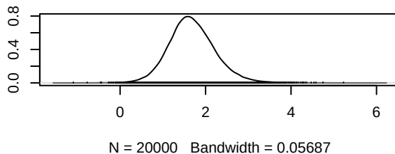
Density of d.Erlotinib.antiangi
