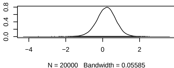
Density of d.Osimertinib.Lazertinib
