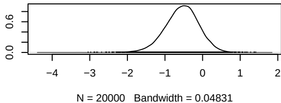
Density of d.Osimertinib.Placebo
