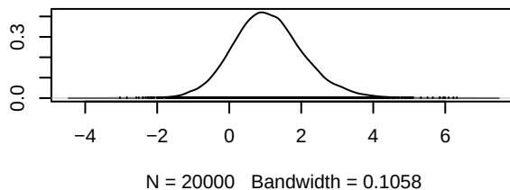
Density of d.Gefitinib.Almonertinib
