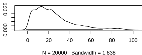
Density of d.Gefitinib.Icotinib
