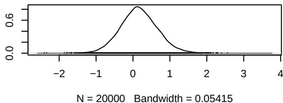
Density of d.chemo.Osimertinib
