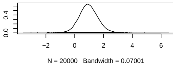
Density of d.Osimertinib.Osimertinib_chemo
