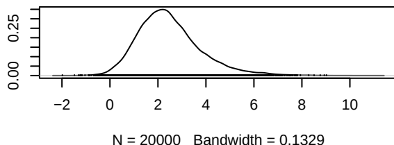
Density of d.Osimertinib.Osimertinib_antiangio
