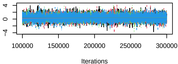
Trace of d.Gefitinib.Furmonertinib
