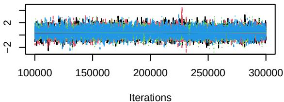
Trace of d.chemo.Erlotinib_chemo
