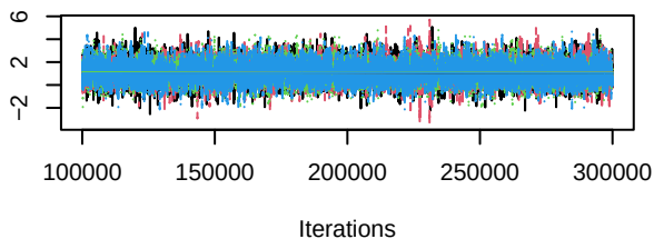
Trace of d.Gefitinib_Erlotinib.Zorifertinib
