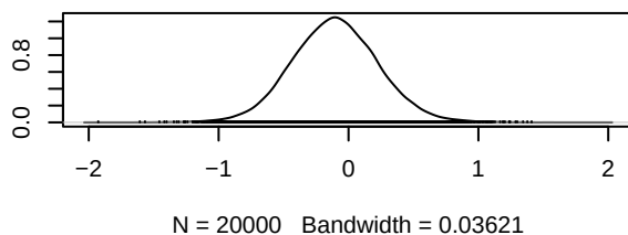
Density of d.chemo.Erlotinib
