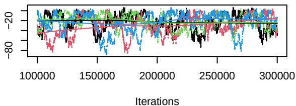
Trace of d.Afatinib.Afatinib_HMGCRi
