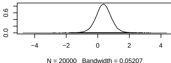
Density of d.Osimertinib.Lazertinib_Amivantamab
