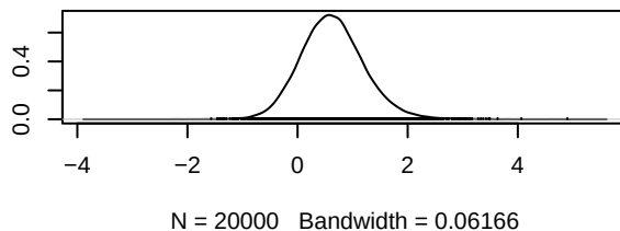
Density of d.Erlotinib.Erlotinib_IGF_1Ri
