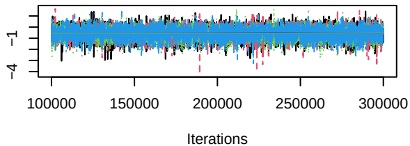
Trace of d.Osimertinib.Placebo
