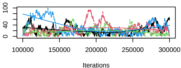
Trace of d.Gefitinib.Icotinib
