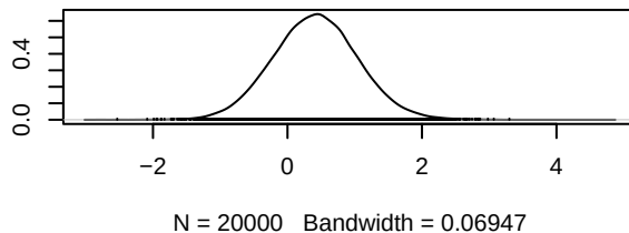
Density of d.chemo.Erlotinib_chemo
