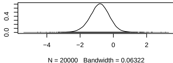
Density of d.Osimertinib.Gefitinib_Erlotinib
