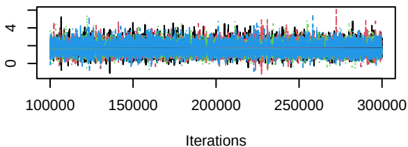
Trace of d.Erlotinib.antiangi
