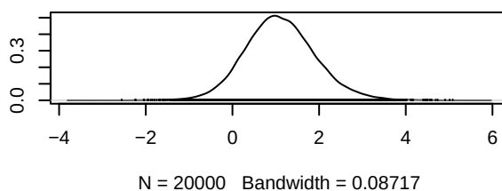
Density of d.Gefitinib_Erlotinib.Zorifertinib
