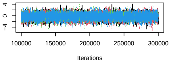
Trace of d.Erlotinib.DHFRi
