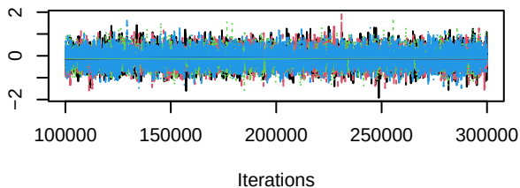
Trace of d.chemo.Erlotinib
