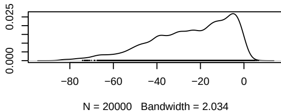
Density of d.Afatinib.Afatinib_HMGCRi
