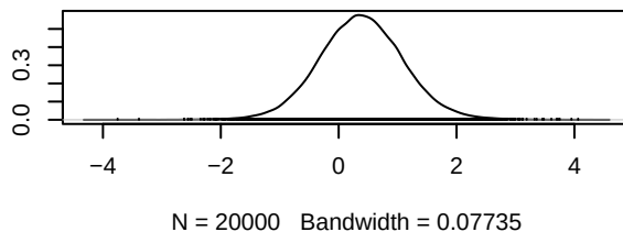
Density of d.Gefitinib.Furmonertinib
